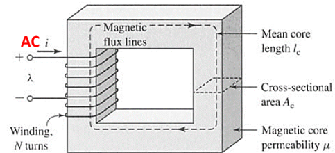
Figure 1.1 Simple magnetic circuit.
