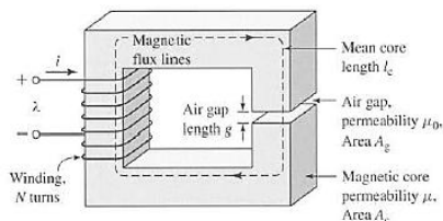
Figure 1.2 Magnetic circuit with air gap.
