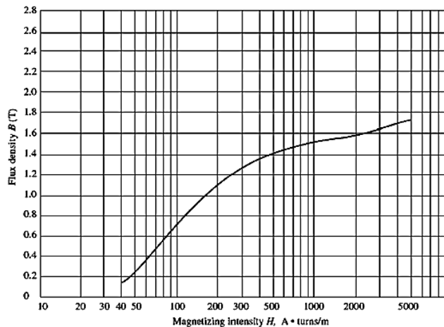
Magnetization curve for steel
