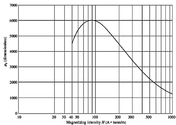
A plot of relative permeability as a function of magnetizing intensity for steel.
