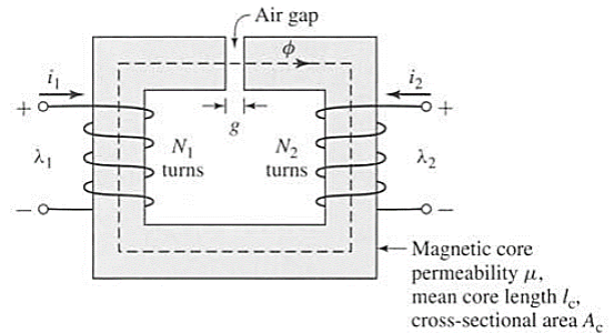
Figure 1.8 Magnetic circuit with two windings.
