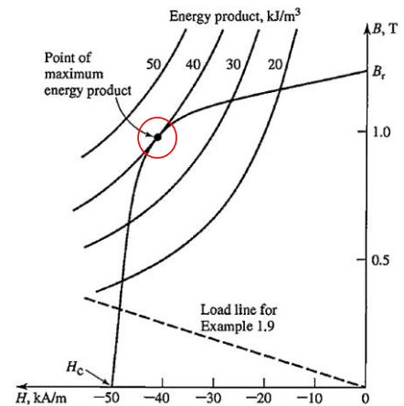
Second quadrant of hysteresis loop for Alnico 5
