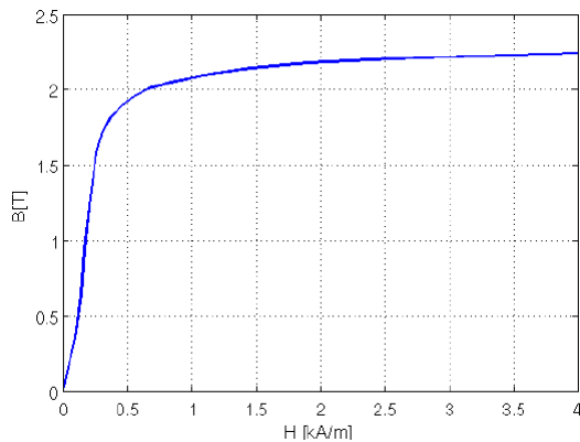
B-H curve for Cobalt-Iron alloy (Vacuumschmelze, 2011)
