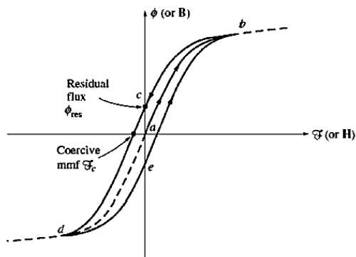
The hysteresis loop
