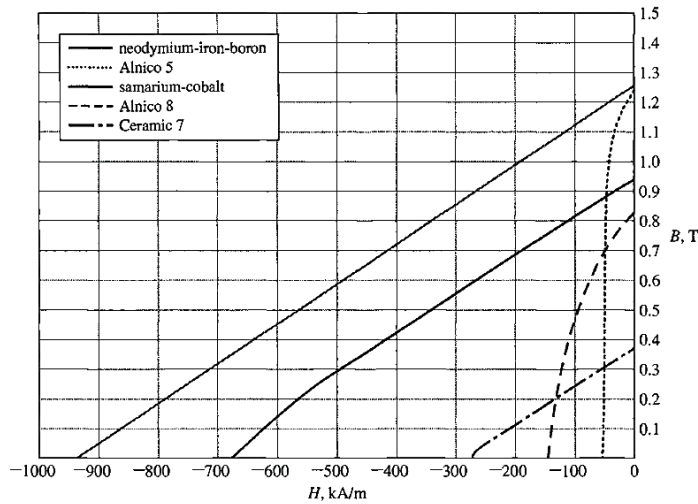
Figure 1.19 Magnetization curves for common permanent-magnet materials.
