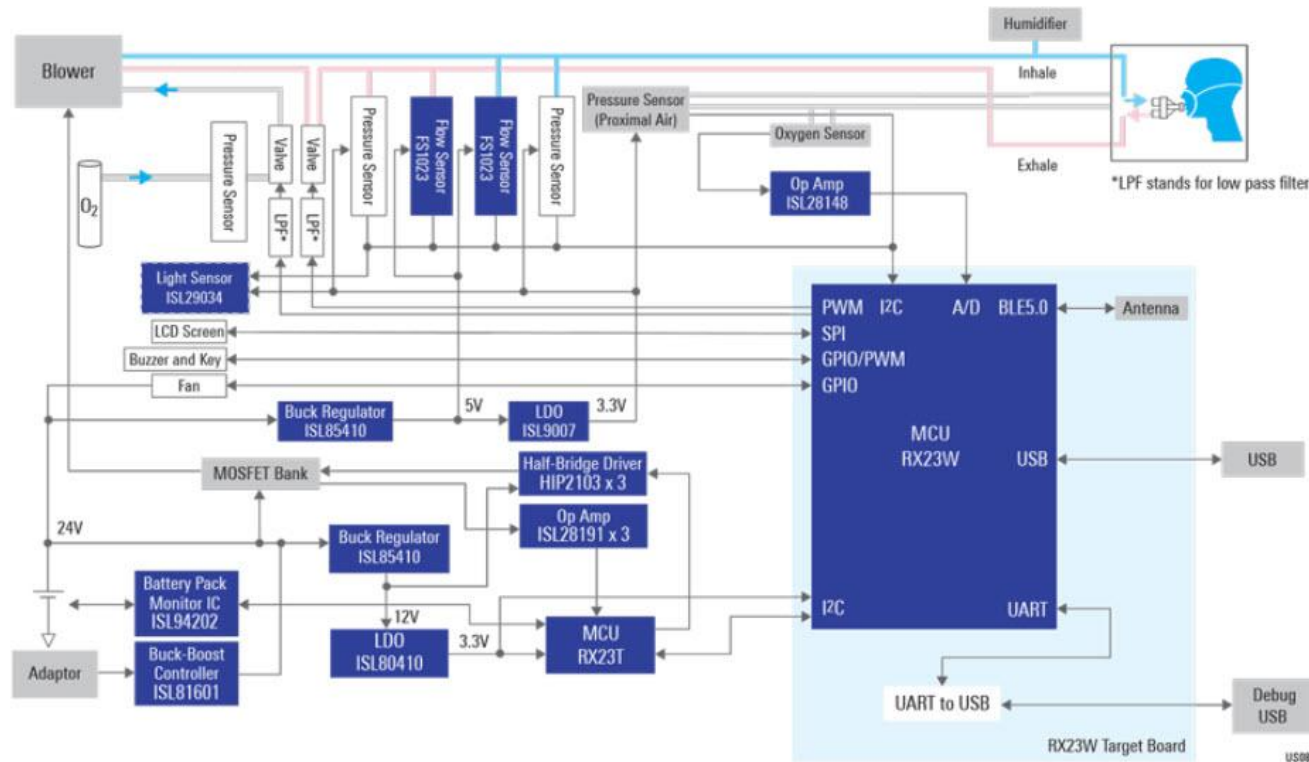
Figure A ventilator system design
