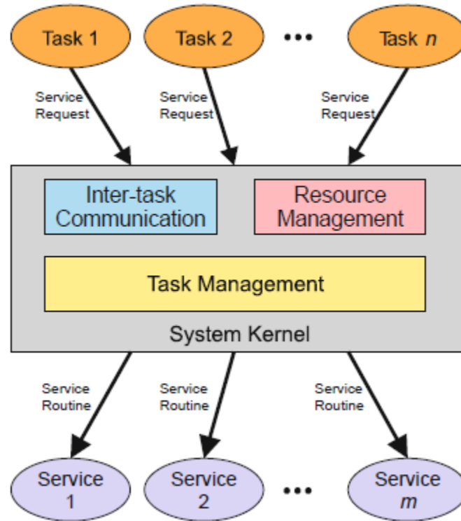
Figure Software structure in an embedded system
