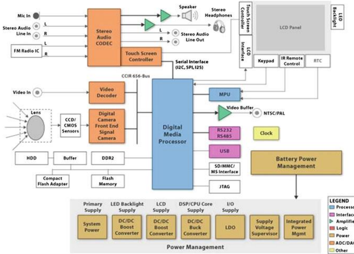
Figure Generic multi-function media player
