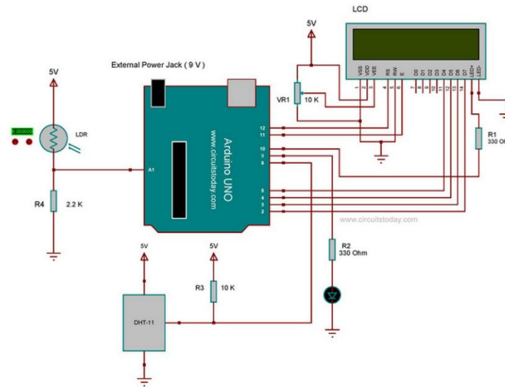
Figure LCD brightness control using Arduino UNO
