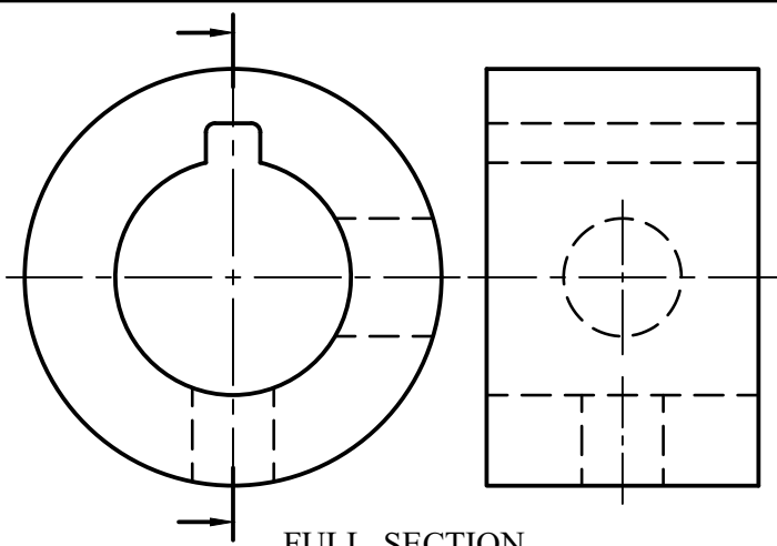
FULL SECTION
