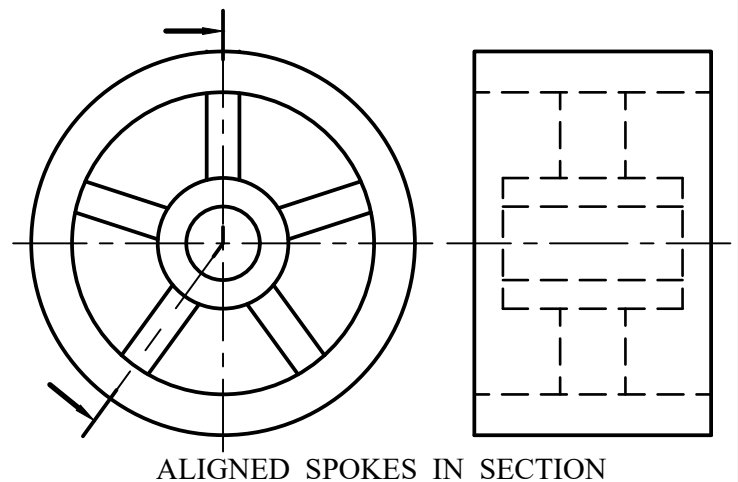
ALIGNED SECTION
