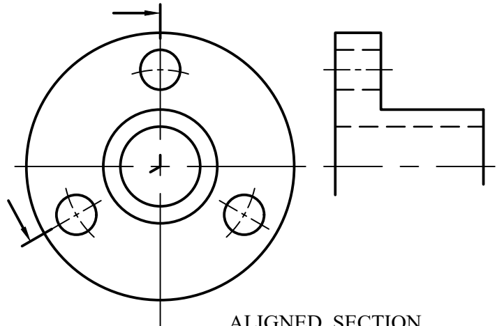
ALIGNED SECTION
