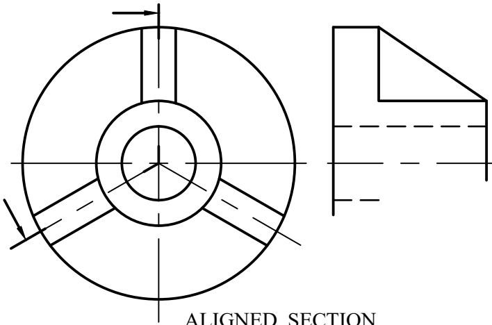
ALIGNED SECTION
