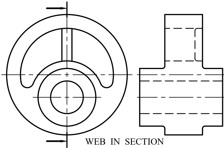
ALIGNED SECTION
