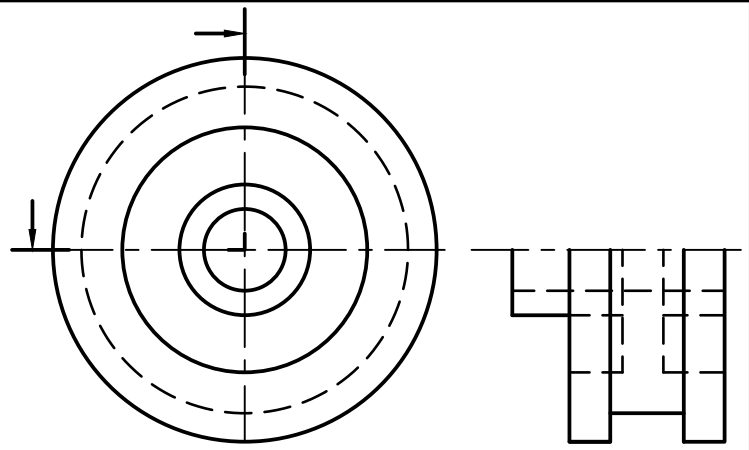
HALF SECTION
