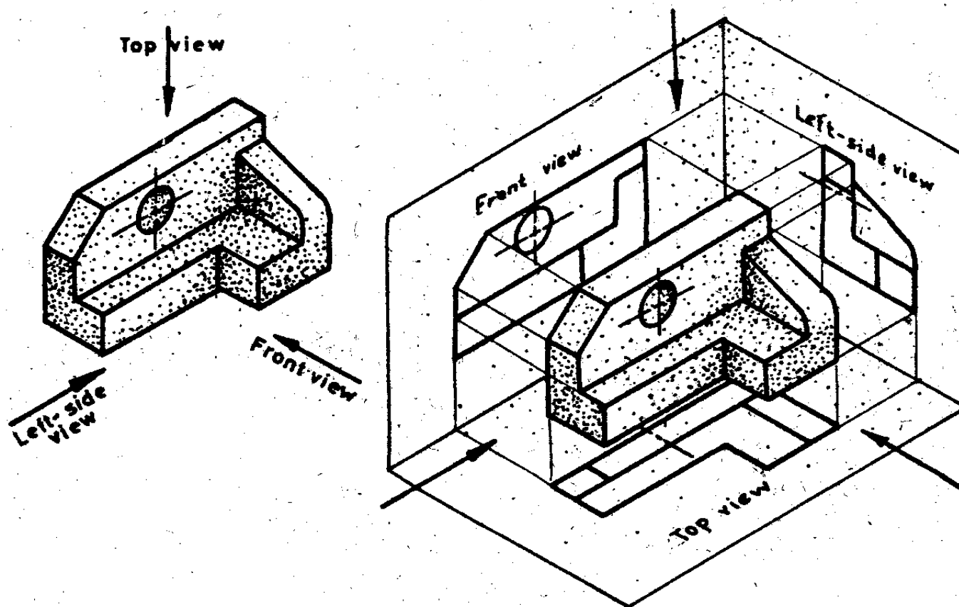
Fig. 4. 23. Object orientation. Use the simplest position. It will give the clearest possible representation and be the easiest to draw.
